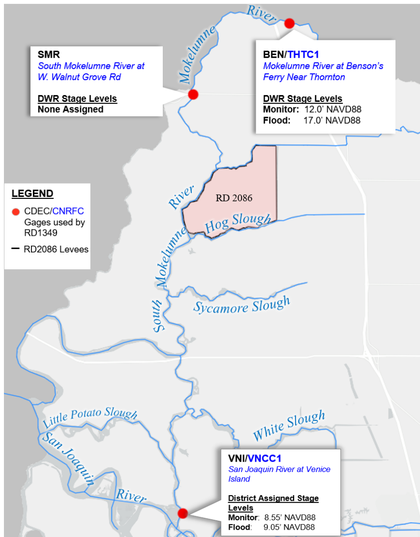
FIGURE 3 | RD 2086 PRIMARY GAGE STATIONS
