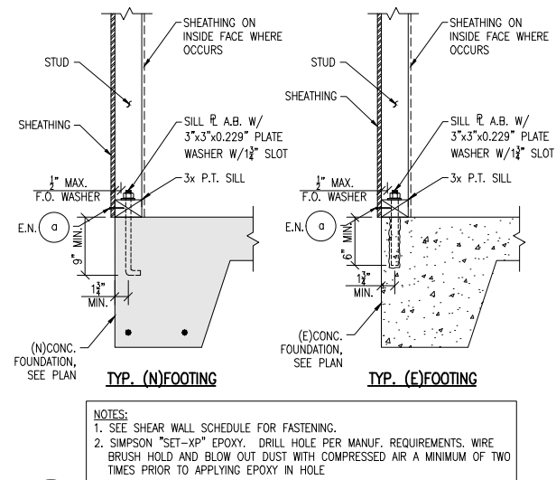
3 TYPICAL ANCHOR BOLT SECTION @ CONCRETE FOUNDATION N.T.S. TDW16A
