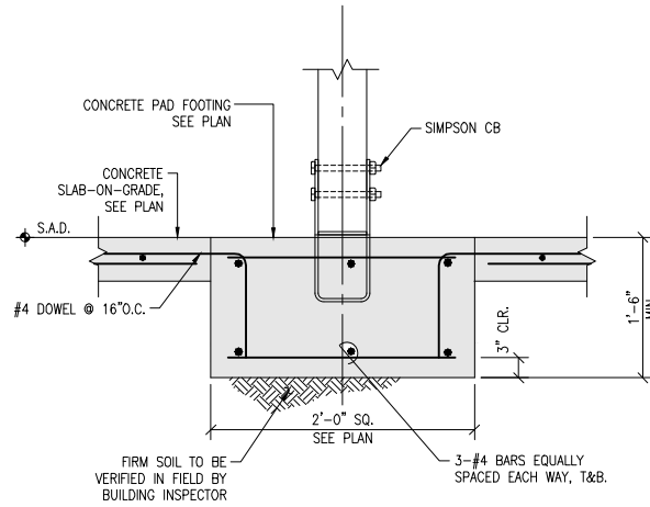
2 TYP WOOD POST ON CONCRETE PAD FOOTING
