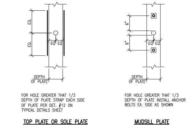
4 DETAIL - HOLES IN PLATES N.T.S. TDW08.dwg
