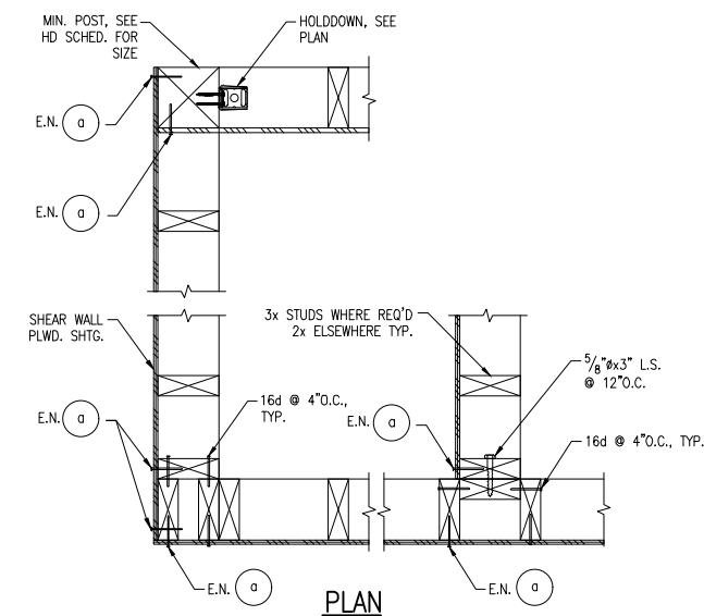
7 DETAIL - SHEAR WALL CONNECTIONS AT INTERSECTIONS & CORNERS N.T.S. TDW03
