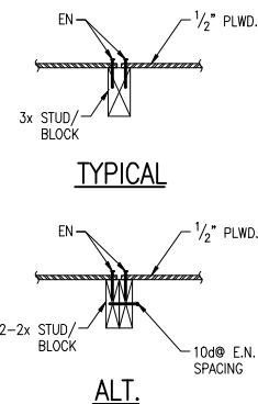
5 ALT. SHEAR WALL PANEL EDGE STUD/BLOCK N.T.S. TDW02A
