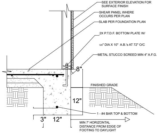
DETAIL 1 (NTS)
