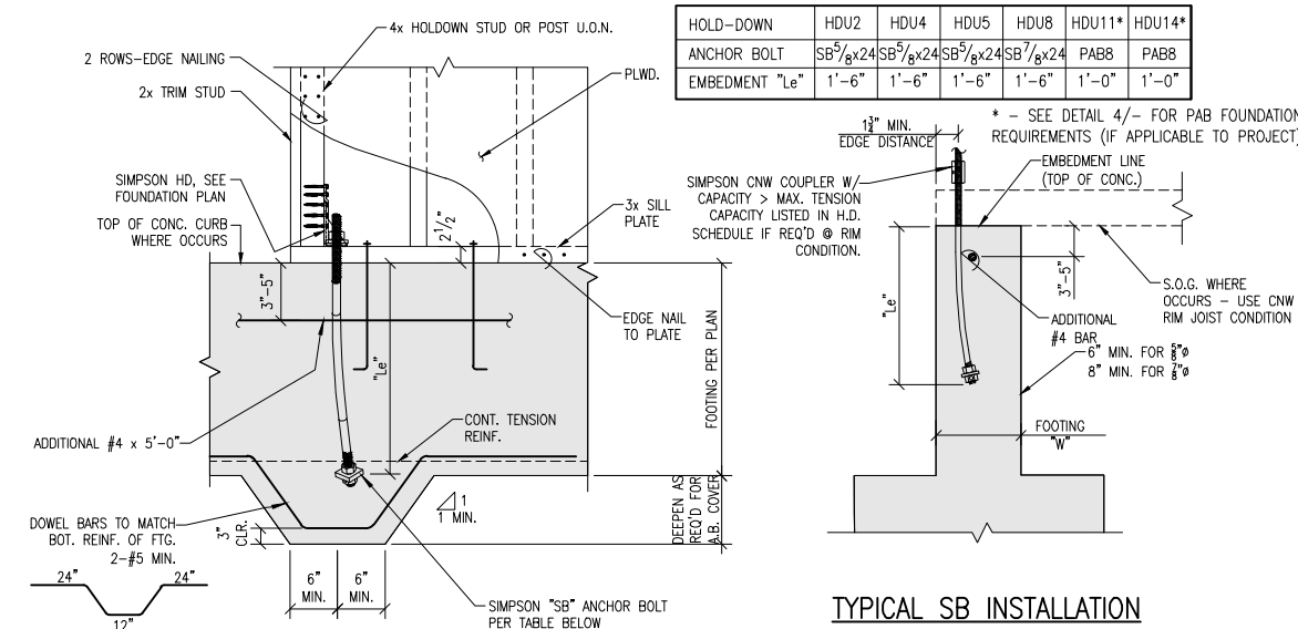
1 TYPICAL HD-TO-(N) FOOTING DETAIL N.T.S. TDW04A.dwg
