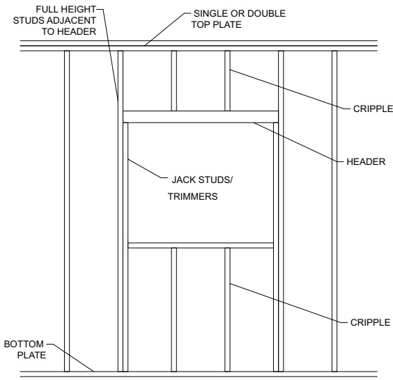
DETAIL 6 (NTS)
