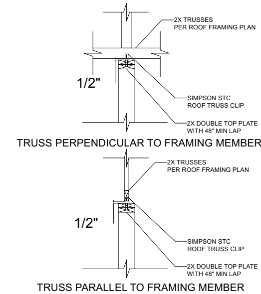
DETAIL 3 (NTS)
