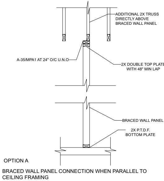
DETAIL 4 (NTS)
