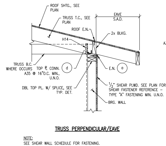
3 TYPICAL SECTION AT ROOF TRUSS - EXTERIOR 1" = 1'-0" TDW22
