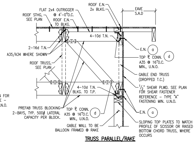
4 TYPICAL SECTION AT ROOF TRUSS - INTERIOR 1" = 1'-0" TDW22
