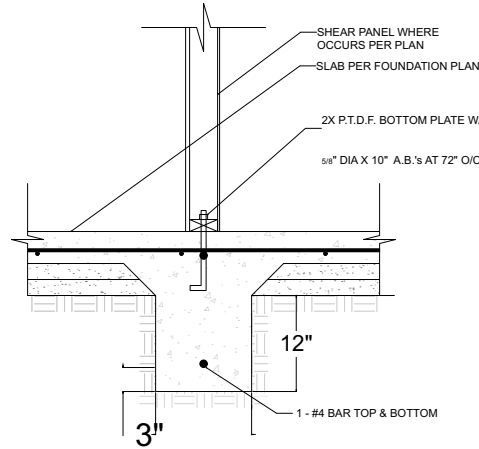
DETAIL 1 (NTS)
