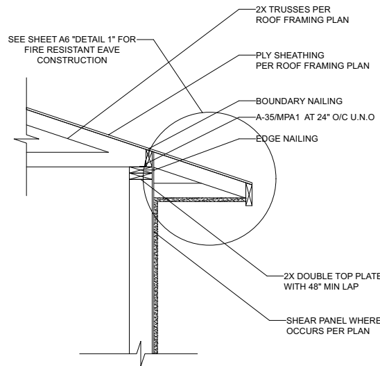
DETAIL 1 (NTS)
